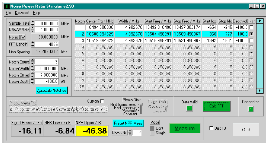
Fig. 27 NPR Microwave Example
