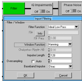
Fig. 4 WinIQSIM Filter Settings
