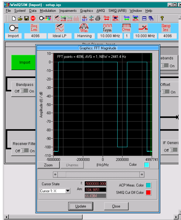
Fig. 28 WinIQSIM Microwave Example
