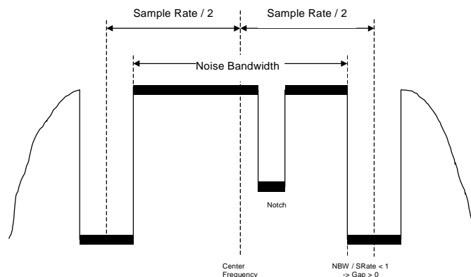
Fig. 10 Noise BW / Sample Rate
