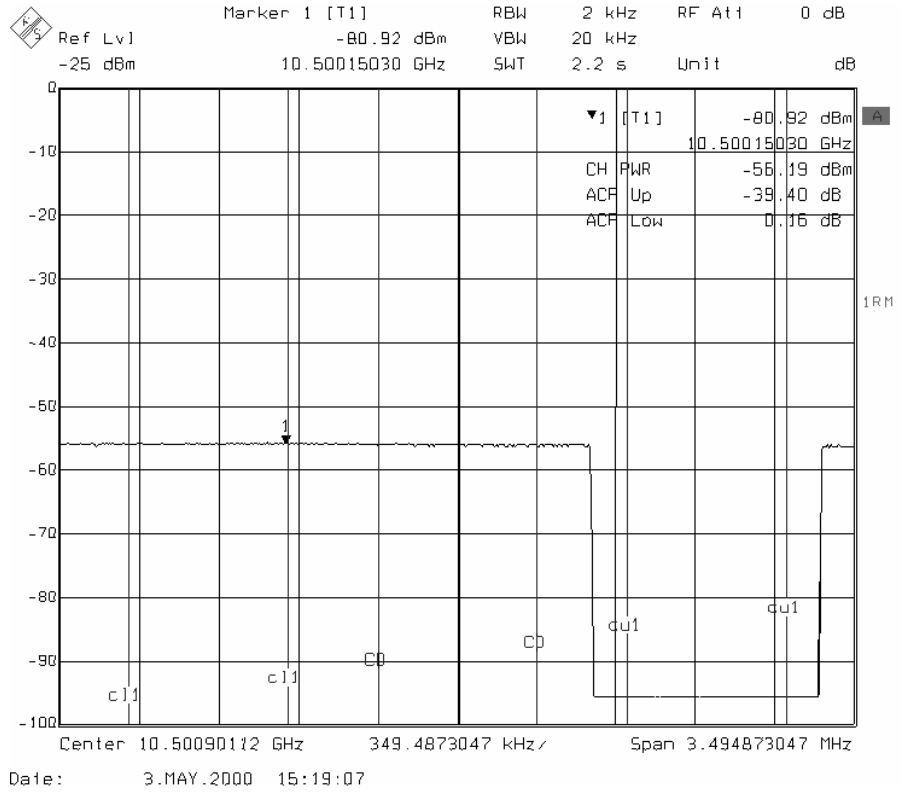
Fig. 29 FSE Microwave Example
