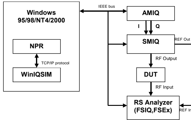
Fig. 1 Connecting Instruments
