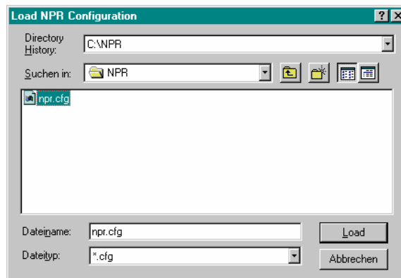
Fig. 20 Load Configuration
