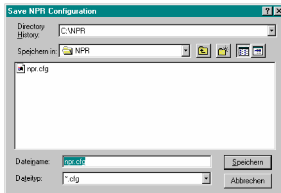
Fig. 21 Save Configuration
