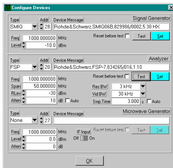
Fig. 22 Device Configuration
