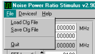
Fig. 19 File Menu
