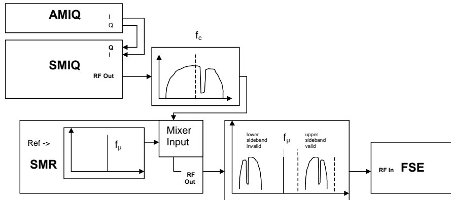
Fig. 26 NPR with Microwaves
