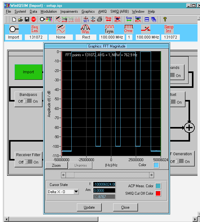
Fig. 6 WinIQSIM Graphic Display
