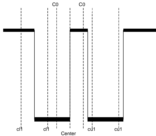
Fig. 25 Correct ACP Readout
